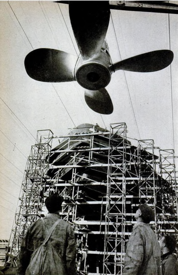
BIGGEST SHIPYARD , the Deutsche Werft, turns out a new ocean-going ship every four weeks. Here an eight-ton propeller is hoisted from ship to hull, which, surrounded by scaffolding (background), sits on one of the yard's seven shipways.
